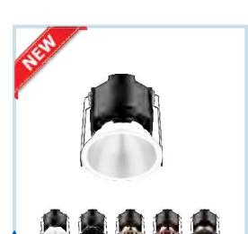
HLR-2516 (7W) Size : Ø62mmx55mm Cut-Out : Ø55mm
