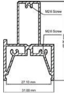
4 wire series
